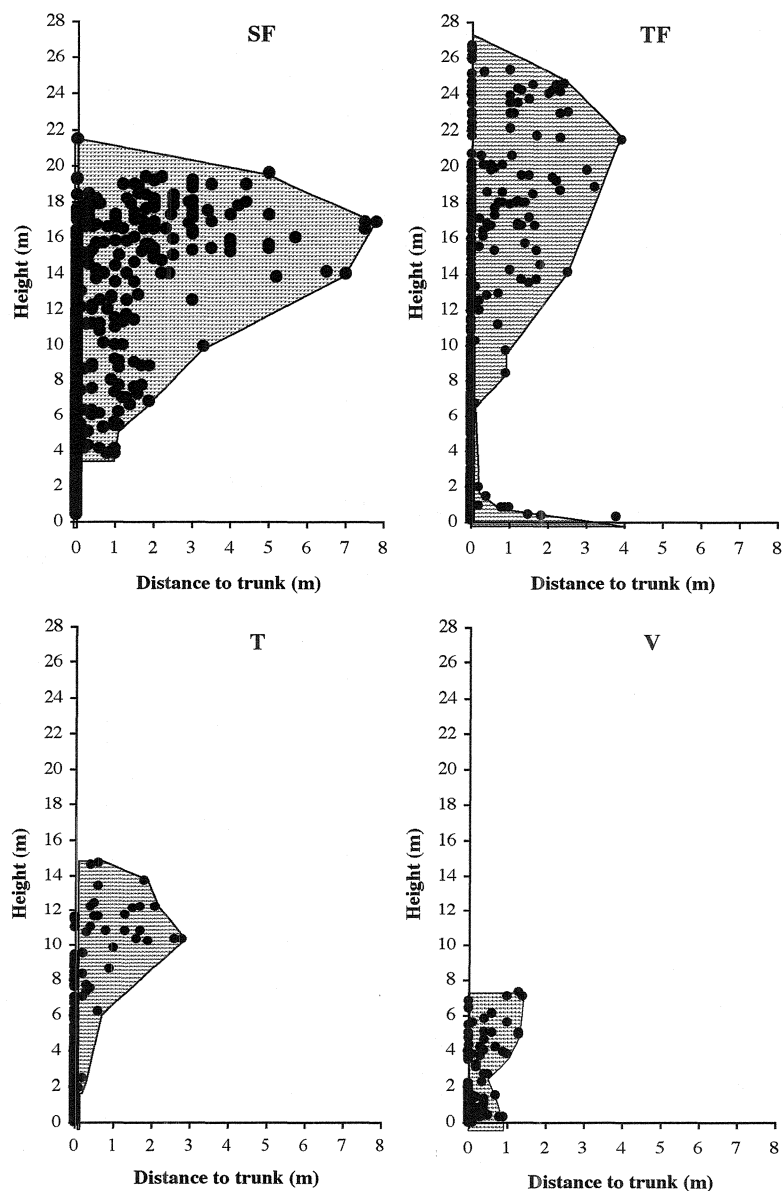
FIGURE 5. Spatial distribution of vascular epiphytes in four forest types of the Serranía de Chiribiquete (Colombia), taking into account the height at which they were found (vertical distance) and distance from the phorophyte trunk axis (horizontal distance).
