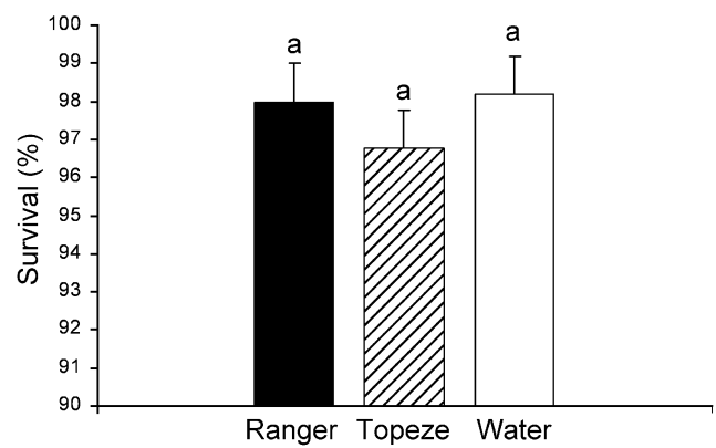
Fig. 1. Survival (%) of Heterorhabditis amazonensis maintained for 5 days in water or exposed to the herbicides Ranger or Topeze. Bars followed by different letters are different by the Scott and Knott test ( P < 0.05 ).
