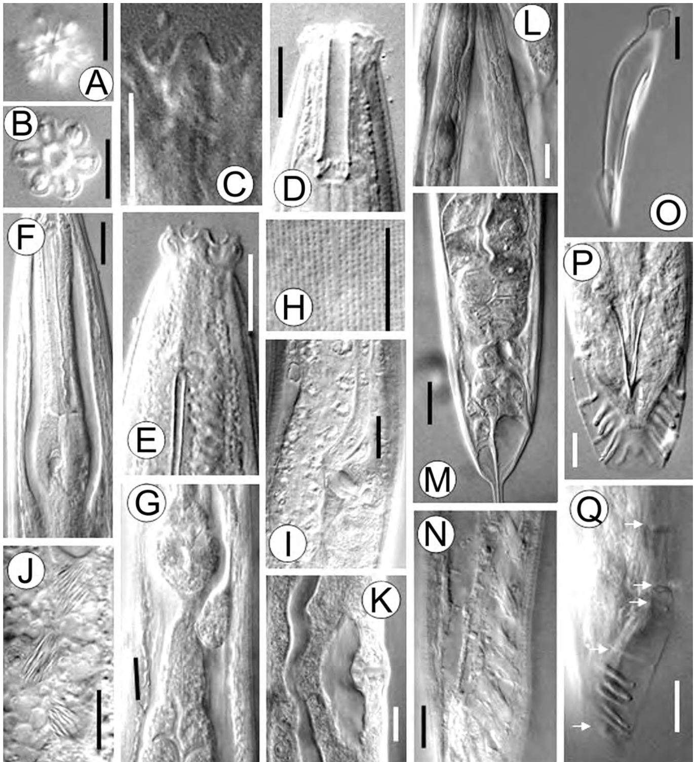
Fig. 2. Pelodera teres (Schneider, 1866). A, B: En face view; C, E: Anterior end (female); D: Anterior end (male); F: Pharyngeal corpus; G: Posterior pharyngeal region; H: Cuticular markings; I: Part of female genital tract; J: Vas deferens with needle-like structures; K: Vulval region (lateral); L: Intra-uterine juveniles; M: Female posterior region showing compactly arranged intestinal cells; N: Male posterior region showing copulatory muscle bands; O: Extracted spicule; P: Male tail (ventral); Q: Male tail (lateral), arrows indicate the less focused papillae. (Scale bar = 10 \mu m).
