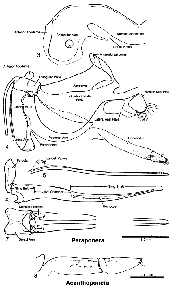
Figures 3-8. Paraponera clavata . 3. Lateral view spiracular plate; dorsal view medial connection. 4. Lateral views quadrante plate, lateral anal plate, oblong plate, gonostylus, triangular plate; dorsal view median anal plate. 5. Lateral view lancet. 6-7. Lateral and ventral views sting, furcula. 8. Acanthoponera minor , lateral view gonostylus.
