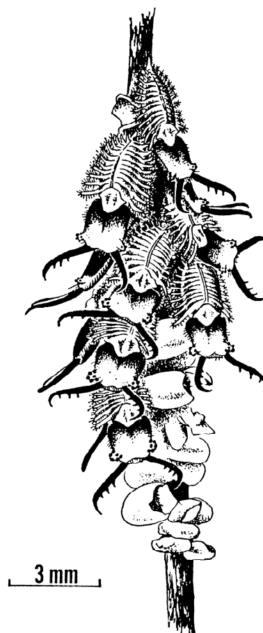
Figure 5. Mass defensive reaction by newly hatched, gregarious larvae of Ascaloptynx furciger (Neuroptera: Ascalaphidae), similar to that of Cassidinae pupae or old larvae of Symphyta (after Henry, 1972).
