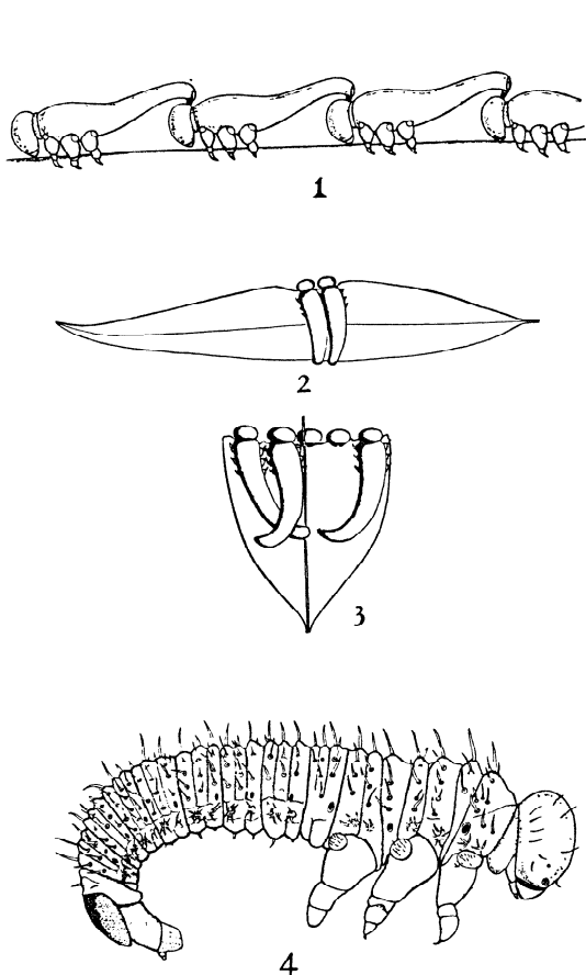
Figure 1-4. Perga dorsalis Leach. 1) Diagrammatic sketch to show a method by which larvae may keep in touch with each other when on the move. 2-3) Diagrammatic sketch of larvae feeding. 4) Full-grown larva, Australia (after Evans, 1934).
