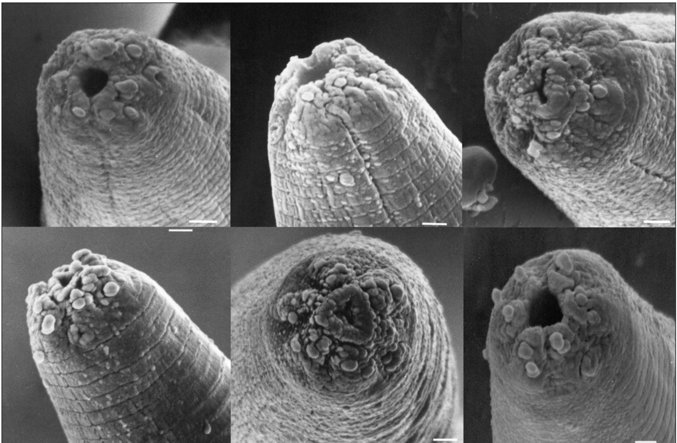
Scanning electron micrographs of lip region of Panagrolaimus individuals
