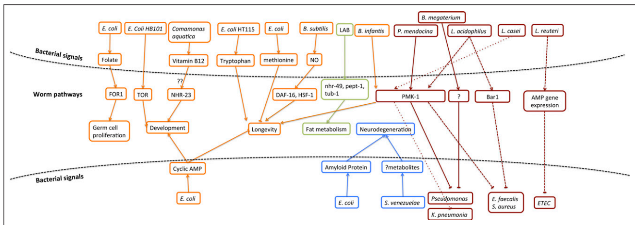
Host-microbe interactions in Caenorhabditis elegans
