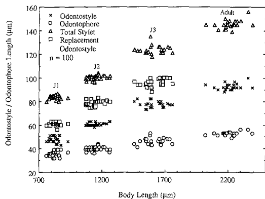
FIG. 2. Scatter diagram plotting the length of all stylet measurements vs. body length for a population of Xiphinema californicum from California.
