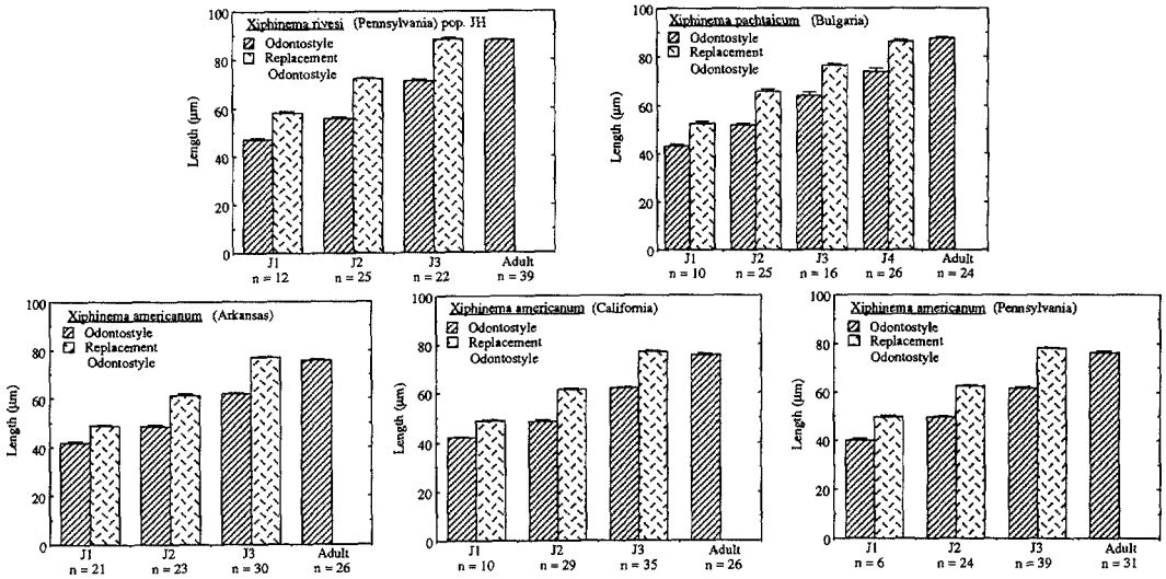
FIG. 3. Length of functional and replacement odontostyle for Xiphinema rivesi , X. pachtaicum , and three populations of X. americanum s. s. (mean \pm SE).
