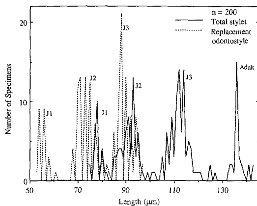
FIG. 1. Frequency distribution of total stylet and replacement odontostyle lengths for a population of Xiphinema rivesi from Pennsylvania.
