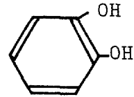
catechol
