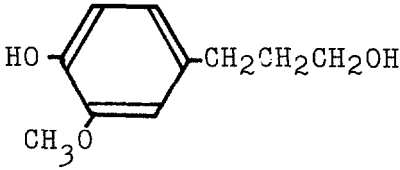
dihydroconiferylalcohol
