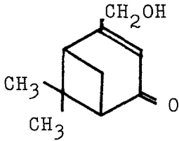
10-hydroxyverbenone
