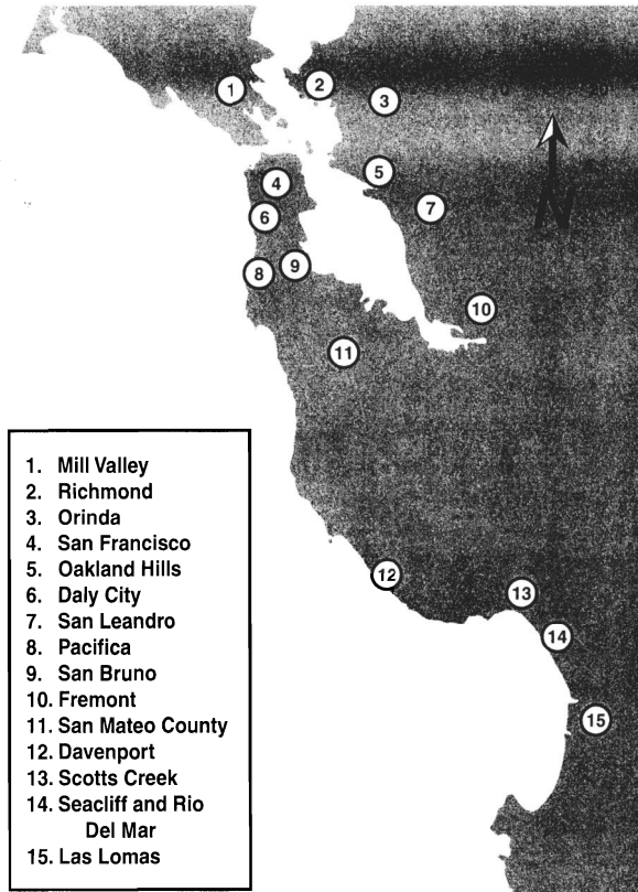
Figure 5. Location of major landslides along the central coast during the 1997–98 ENSO winter. All of the landslides were a result of the high precipitation during the 1997–98 winter; wave erosion played a part in the failure of the coastal bluffs only in Pacifica. Data from the California Department of Conservation's Division of Mines and Geology ( http://www.consrv.ca.gov/dmg/ ).
