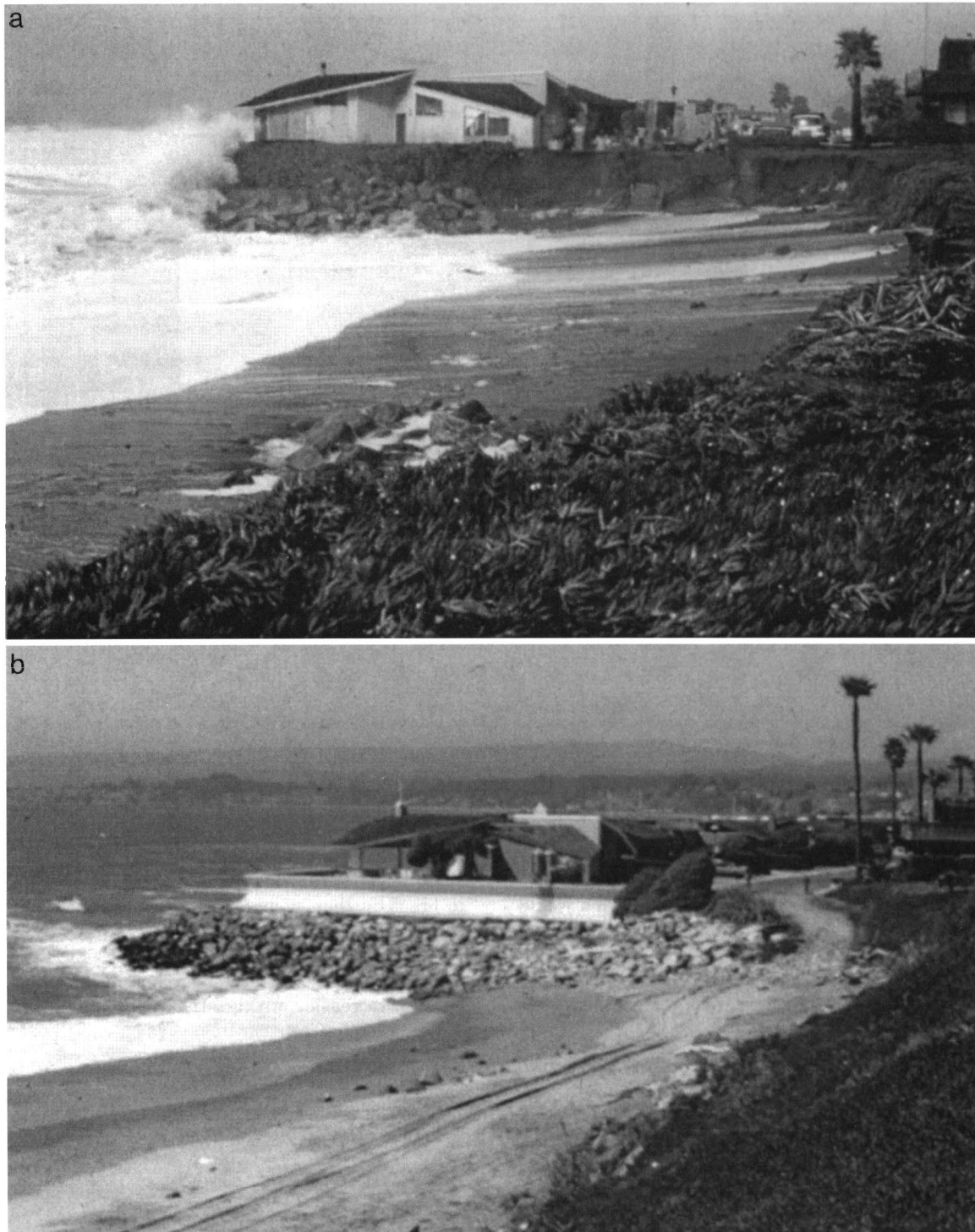
Figure 11. Changes in the construction and the effectiveness of coastal protection structures along Via Gaviota in Aptos-Seascape during early (a) 1983, and (b) 1998. Following the storms of early 1983, the rip-rap revetment was removed, a new curved-face concrete seawall was placed upon steel piles driven to refusal, and the rip-rap was then placed back at the toe of the seawall to provide additional protection. None of the houses along Via Gaviota reported wave-induced damage during the 1997–98 winter.
