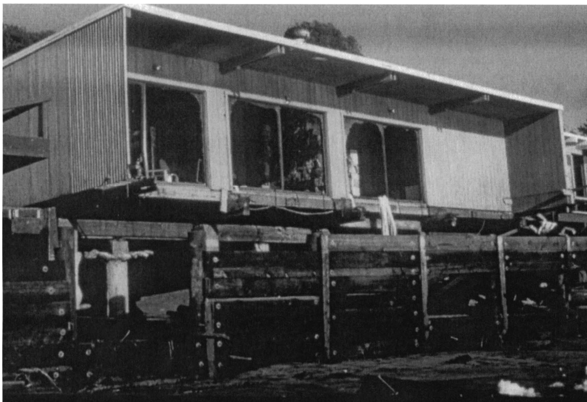
Figure 2. Damage to a house and timber seawall along Beach Drive in northern Monterey Bay resulting from the storms of early 1983. The seawall was battered and breached by waves and debris, allowing over 2 m of fill behind the wall to be scoured, undercutting the structure and threatening the structural support system.
