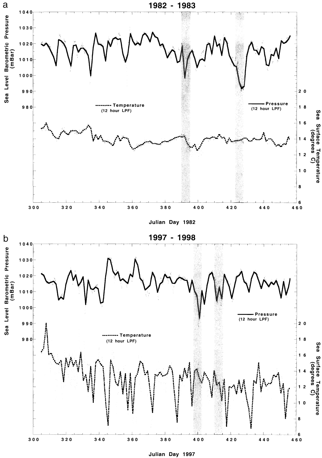
Figure 7. Fluctuations in sea level barometric pressure and sea surface temperature from NOAA buoy #46026 during the (a) 1982–83 ENSO event, and (b) the 1997–98 ENSO event. The dark lines represent 12-hour low-pass-filtered signals while the dots represent hourly data values. The grey bands denote the periods when the most intense storms struck the central coast. The sharp drops in sea surface temperature during the 1997–98 winter typically follow storms incident from the northwest with high sustained wind velocities.
