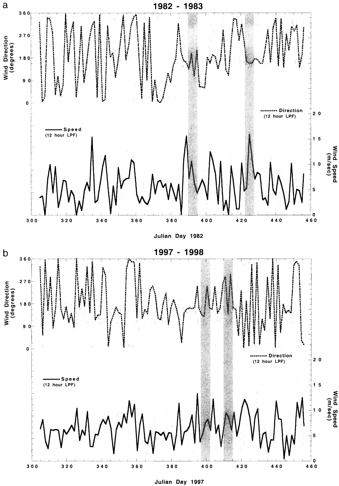
Figure 6. Fluctuations in wind direction and velocity from N.O.A.A. buoy #46026 during the (a) 1982–83 ENSO event, and (b) the 1997–98 ENSO event. The grey bands denote the periods when the most intense storms struck the central coast. Note the correlation between the higher wind velocities and the more southwesterly directions during the major 1982–83 storms as compared to the 1997–98 storms.
