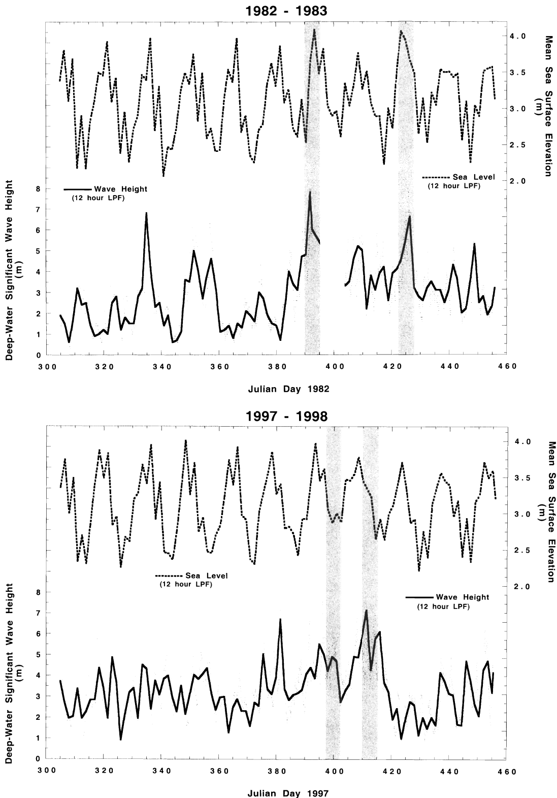
Figure 8. Fluctuations in the sea surface elevation at Monterey Harbor and wave height from N.O.A.A. buoy #46026 during the (a) 1982–83 ENSO event, and (b) the 1997–98 ENSO event. The dark lines represent 12-hour low-pass-filtered signals while the dots represent hourly data values. The grey bands denote the periods when the most intense storms struck the central coast. Note the coincidence of large waves and spring tides in 1982–83, while the largest waves in 1997–98 struck the central coast during neap tides.
