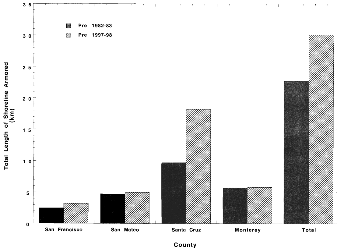
Figure 10. Distribution of coastline protection structures along central California and the increase in the number of structures between the 1982–83 and 1997–98 ENSO winters. Overall, there was a 30% increase in armoring along the central coast following the 1982–83 ENSO event.
