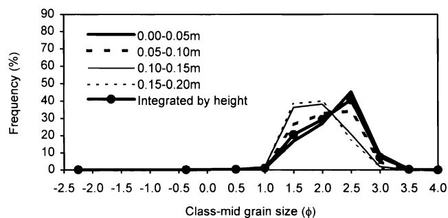
Figure 13. Example of the distribution of grain size with height (trap T3, 21 October 1996, 10:30-11:00).
