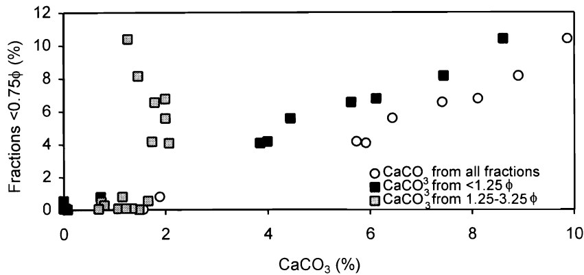
Figure 6. CaCO 3 content versus fractions <0.75 φ (>0.600 mm) for the nourishment sand samples displayed in Fig. 5.
