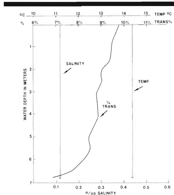
Figure 8. A temperature, salinity, and transparency profile obtained from a research vessel 24 hours after a cold front passage. The plot shows the destratified state of Atchafalaya River Discharge waters in the bay in terms of temperature and salinity with a subtle (3%) change in the transmittance (suspended sediment concentration) profile.
