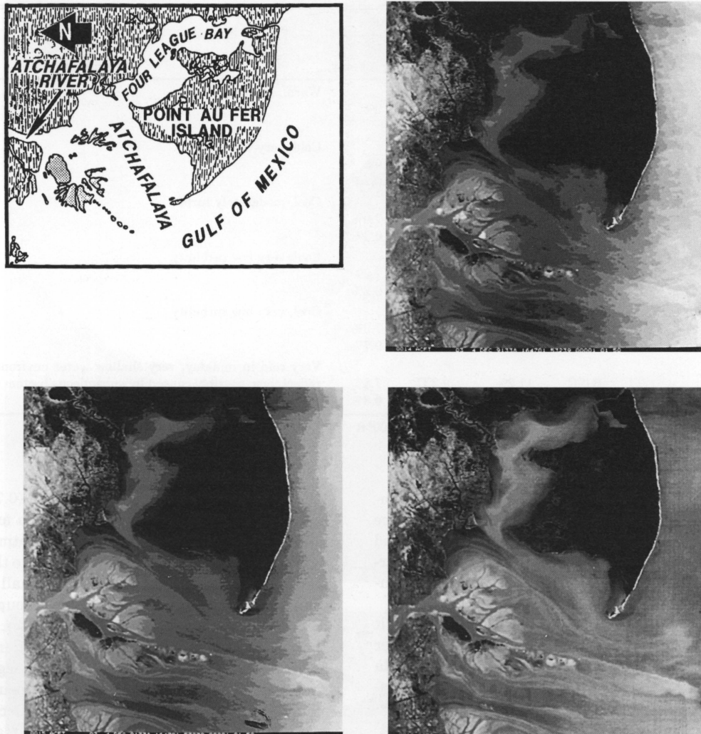
Figure 3. (a) Image location map; (b) MAMS uncorrected band 3 (.56 \mu\text{m} ) imagery; (c) after sunglint removal; (d) after atmospheric scattering removal, leaving an image of scaled water leaving reflectance ( x = 500 \cdot R ). Sunglint correction is not attempted over land surfaces.
