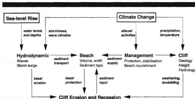
Figure 1. Summary of factors influencing cliff erosion.
