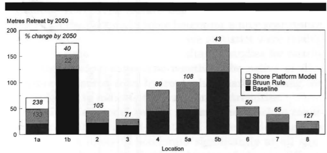
Figure 3. Extrapolations of cliff recession indicating the potential effects of sea-level rise superimposed upon baseline conditions. Note the lower predictions of the modified Bruun Rule which models the capacity of cliff sediments to build up the shore profile.
