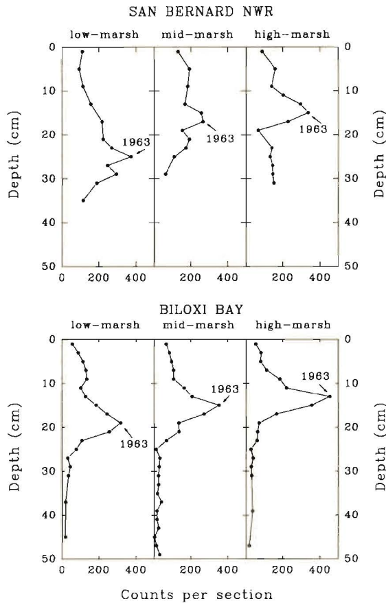
Figure 4. Profiles of 137 Cs activity for high, mid and low-marsh cores from San Bernard NWR (top) and Biloxi Bay (bottom). Peaks in 137 Cs activity correspond to 1963.
