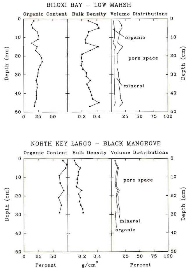
Figure 3b. Profiles of organic content, bulk density, and sediment volume distributions for cores from the low marsh at Biloxi Bay (top) and from the black mangrove station at North Key Largo (bottom).
