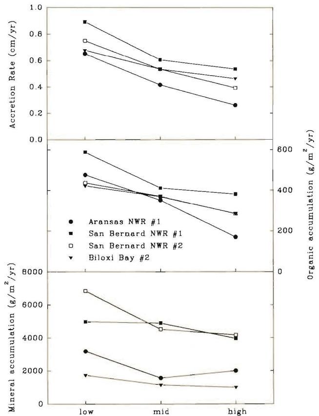
Figure 5. Rates of vertical accretion (top), organic accumulation (middle), and mineral accumulation (bottom) from transects across the marsh. Data are for complete transects from salt marsh sites only.
