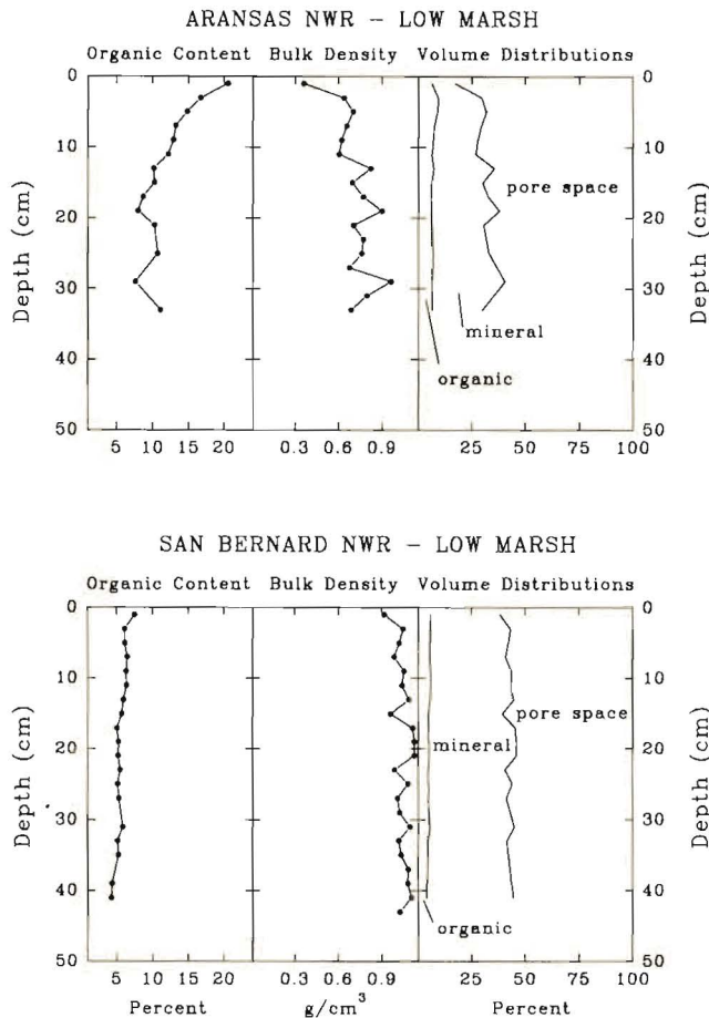
Figure 3a. Profiles of organic content, bulk density, and sediment volume distributions for cores from the low marsh at Aransas NWR (top) and San Bernard NWR (bottom).
