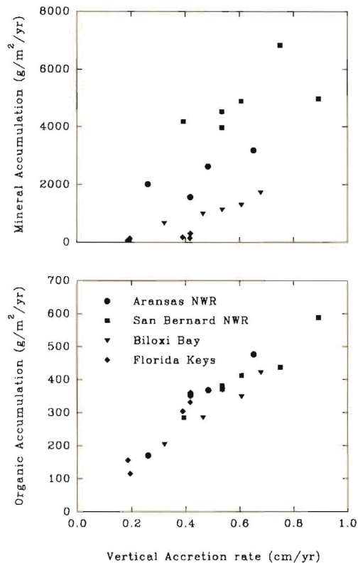
Figure 7. Correlation of vertical accretion rates with mineral accumulation rates (top) and organic accumulation rates (bottom) for all cores.
