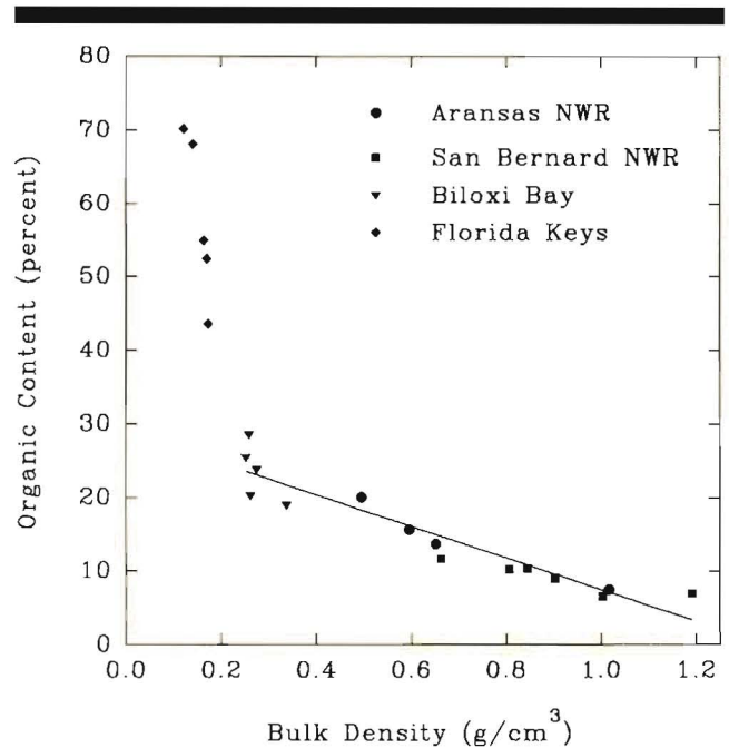
Figure 2. Organic content and sediment bulk density for the top 10 cm of cores collected from all sites. Solid line indicates correlation for salt marsh sites only ( r^2 = 0.87 ).
