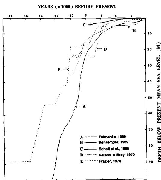
Figure 2. Late Wisconsinan and Holocene sea-level records, Southeastern United States and Barbados.
