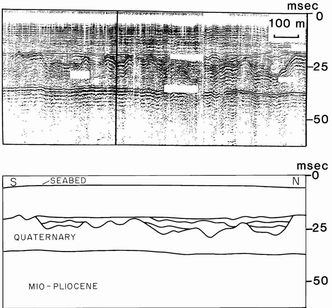
Figure 8. Sub-bottom seismic data from western Apalachicola Bay, showing a paleochannel of the late Holocene Apalachicola River. Two-way travel time in milliseconds is shown at right. Full vertical scale is approximately 60 meters. Location of profile is indicated in Figure 1.
