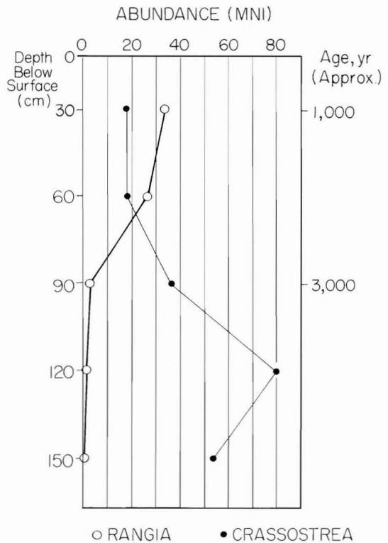
Figure 4. Van Horn Creek shell midden (8Fr744) mollusk abundance profile. MNI = minimum number of individual mollusks per standard 4-liter sample for each 15 cm level. Dates indicated are based on the presence of ceramics of known age. Location of midden site is indicated by "VH" in Figure 7. (Data and figure from K.J. Walker, Florida Museum of Natural History.)
