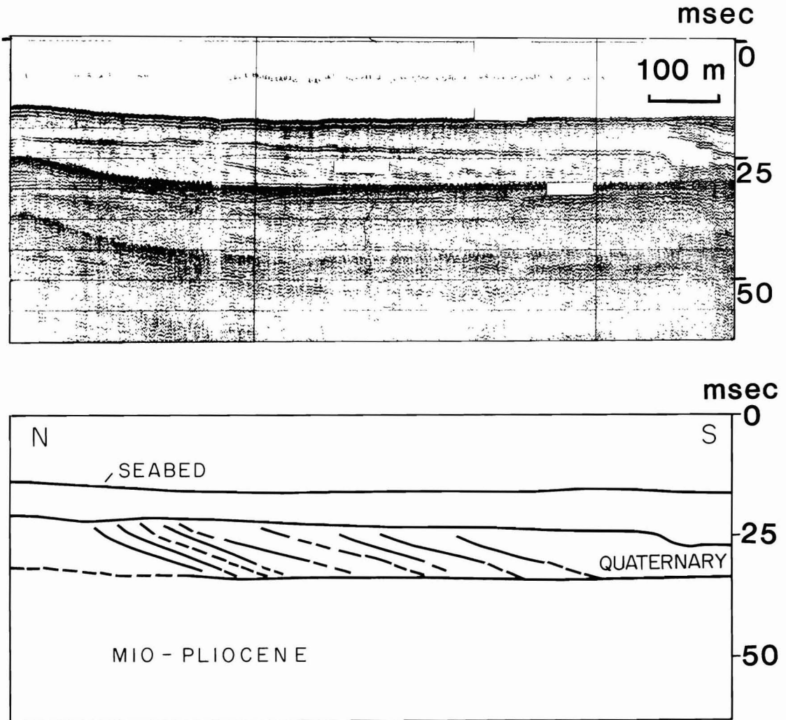
Figure 9. Sub-bottom seismic data from east side of Cape St. George Shoal, showing paleo-deltaic deposits of the Apalachicola River. Two-way travel time in milliseconds is shown at right. Full vertical scale is approximately 60 meters. Location of profile is indicated in Figure 1.
