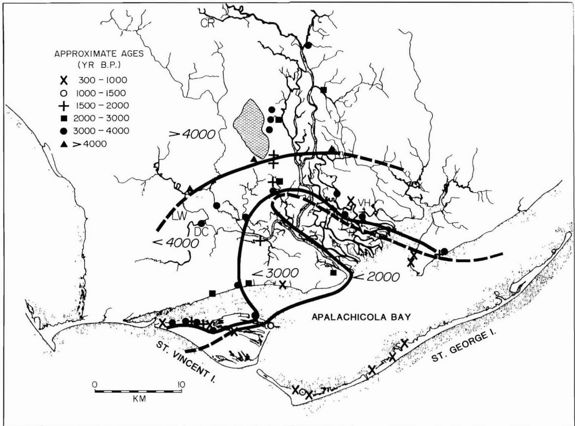
Figure 7. Age distribution of archaeological sites in the lower Apalachicola River valley. Symbols indicate approximate known age of oldest artifacts found at all dated sites within the lower watershed. Contours show maximum age of enclosed sites, indicating close connection between delta migration and human settlement pattern. Contours are dashed where uncertain. Abbreviations: (CR) Chipola River, (DC) Depot Creek shell midden, (LW) Lake Wimico, (VH) Van Horn Creek shell midden. Patterned area northwest of modern Apalachicola Delta is "late Pleistocene" delta, as mapped by SCHNABLE (1966).
