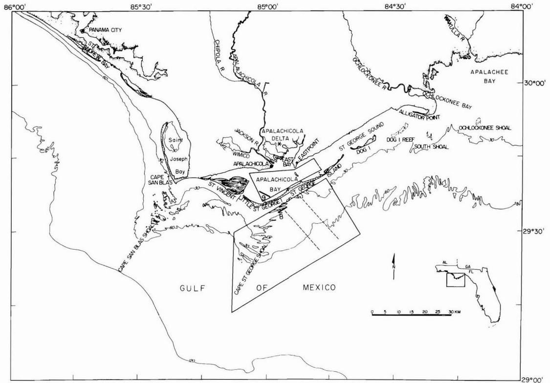
Figure 1. Apalachicola Delta region. Bathymetry in feet. Outlined areas are locations of high-resolution seismic surveys. Pattern on St. Vincent Island shows general trend of beach ridge sets. Dashed lines show trend of large Apalachicola paleochannel system, as described in text. Locations of seismic lines in Figures 8 and 9 are indicated by numbers. Location of Van Horn Creek shell midden is shown by symbol under Apalachicola Delta label.
