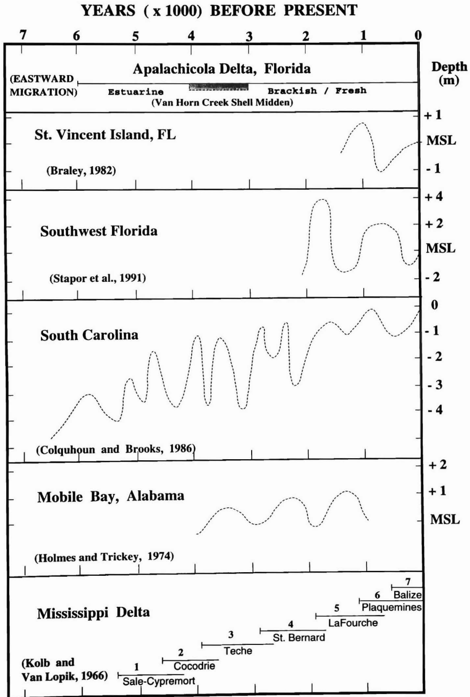
Figure 3. Composite evidence of late Holocene sea-level fluctuations, northern Gulf of Mexico. The Apalachicola Delta chronology indicates the approximate date of initiation of the modern delta. Also shown is the period of environmental transition (stippled pattern) for the vicinity of the Van Horn Creek shell midden (location shown in Figure 1). All sea-level curves are discussed in the text. All dates are in uncorrected radiocarbon years BP. [Notes: (1) The vertical datum for the South Carolina curve is "meters below present high marsh surfaces." Relation to mean sea level is uncertain. (2) The late Holocene deltas of the Mississippi are arranged chronologically; no elevation difference is implied.]
