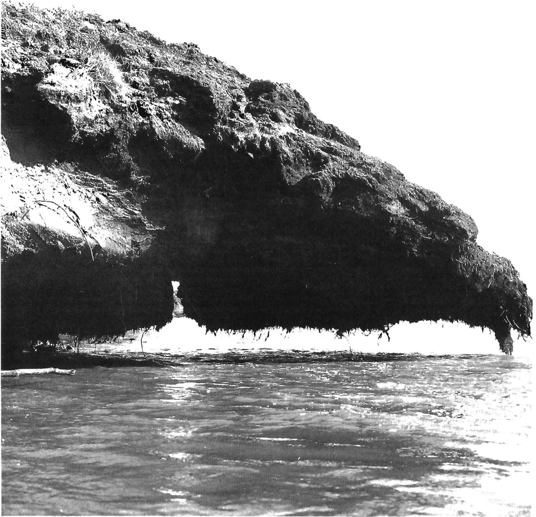
PHOTO 59. Thermoerosional niche in peat bank in the Colville River, Alaska. Note the ice wedge that has begun to thaw from beneath.
