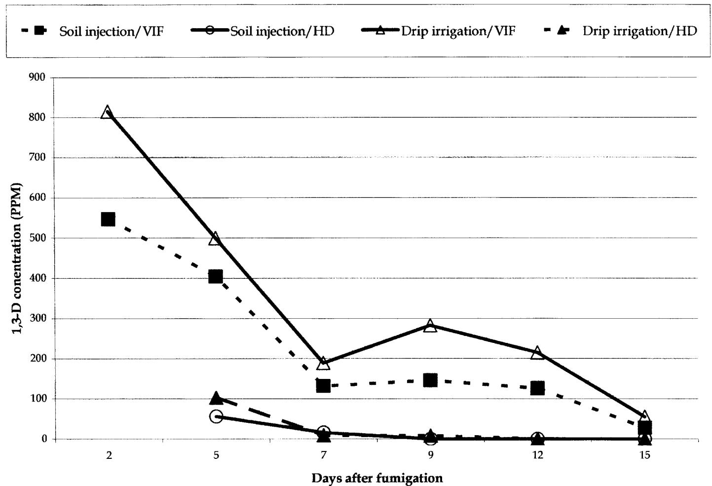
Fig. 1. Effect of soil fumigant, method of application and mulch type on gas concentrations of 1,3-D at the bed center over time.
