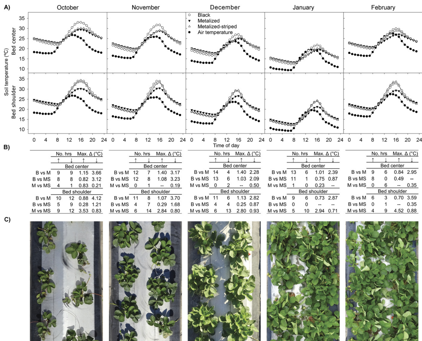
Fig. 2. (A) Average hourly root-zone temperatures at a 10-cm depth for the bed center and bed shoulder. (B) Tables showing the number of hours of statistically significant differences as well as the maximum change in temperature ( \uparrow = increased temperature; \downarrow = decreased temperature) for each comparison shown on the left (B = black mulch; M = fully metalized mulch; MS = metalized-striped mulch). Comparisons are given as the second mulch type relative to the first mulch type. (C) Representative photos of the growth stage of 'Florida Radiance' are given for each month.
