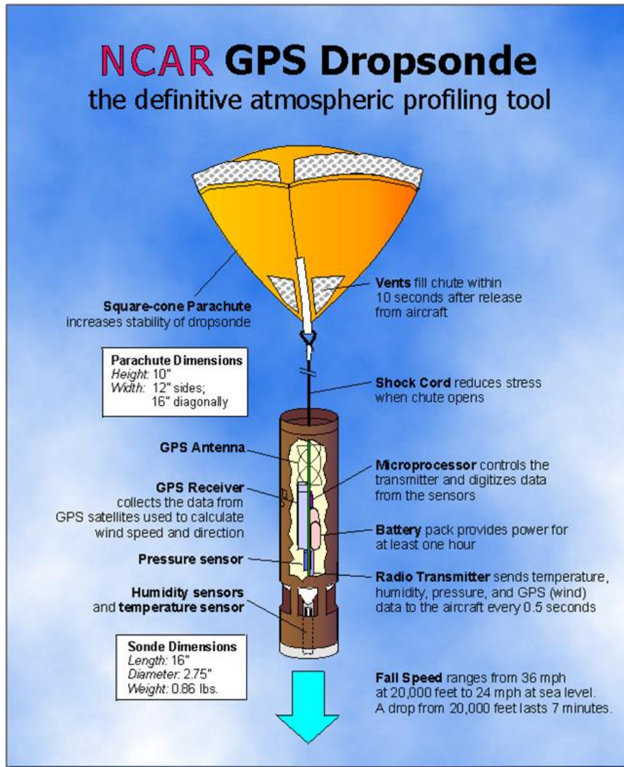
Figure 9: GPS Dropsonde
