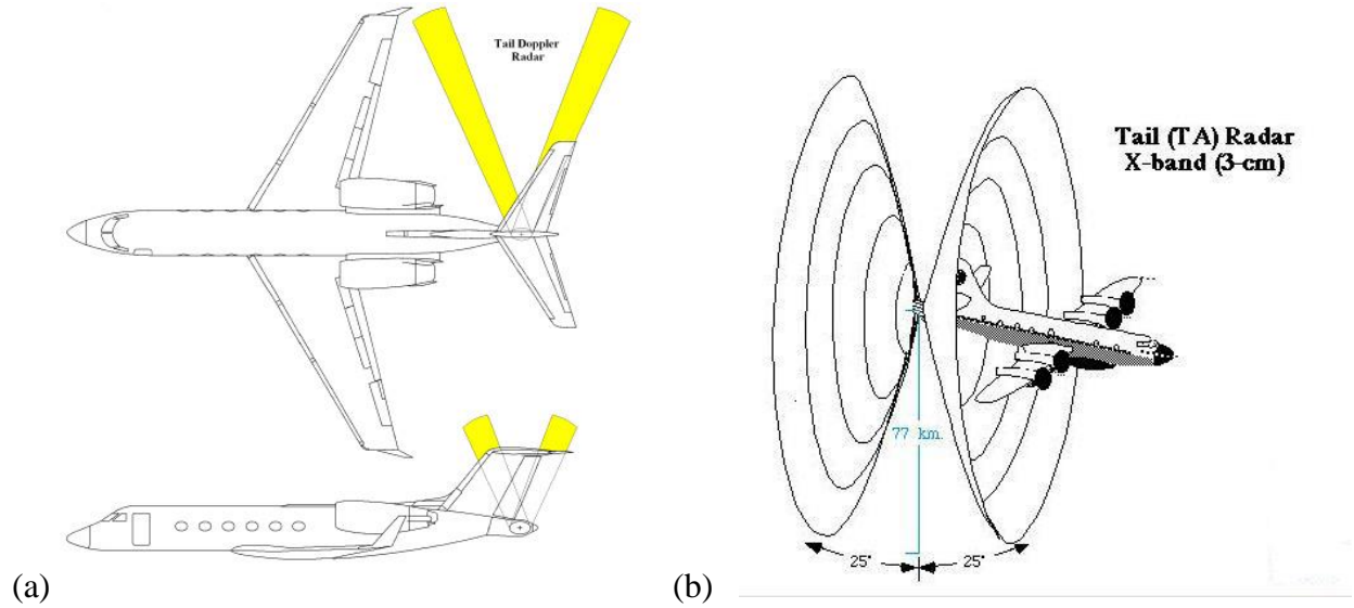
Figure 7: The Tail Doppler Radar's Location on the (a) NOAA G-IV and the (b) NOAA WP-3D Orion
