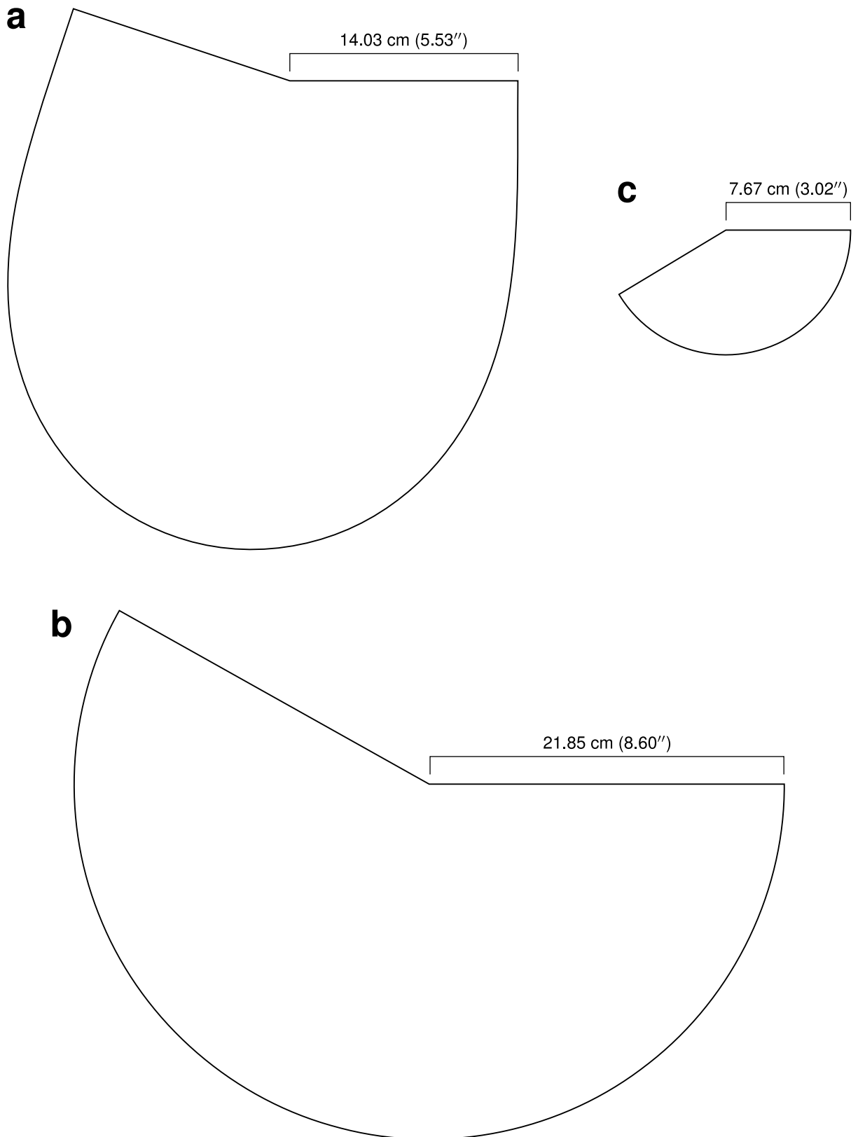
Fig. S1. Patterns for fabricating trap cones from aluminum window screen: a) side cone of trap box; b) top cone of trap box; and c) cone in jar assembly.
