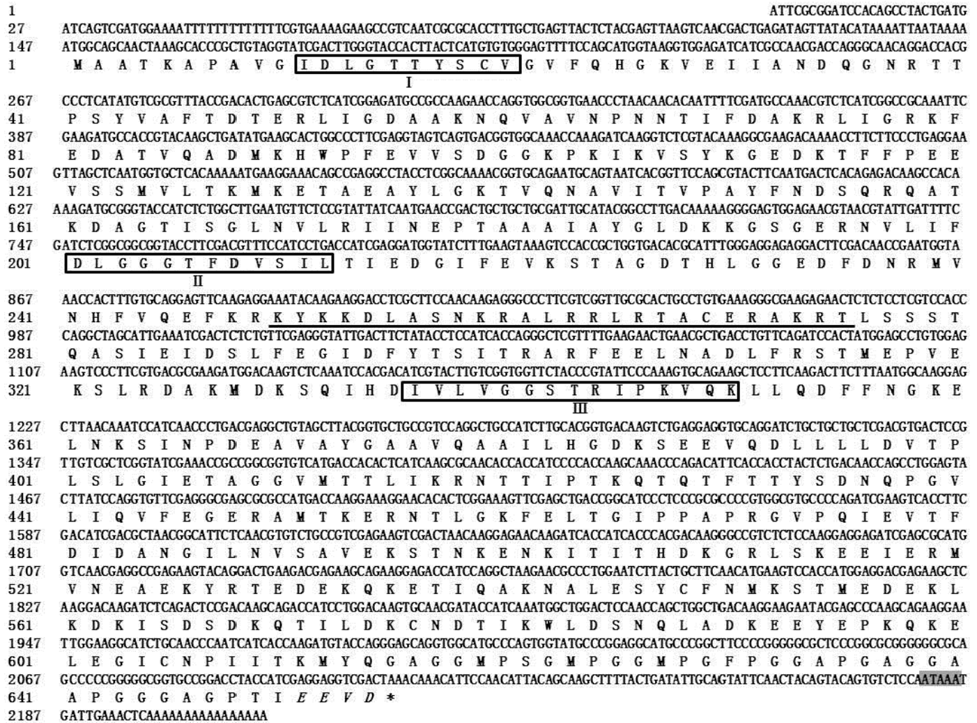
Fig. 2. Nucleotide and deduced amino acid sequences of the Xc-HSP70 gene. The signature sequences of the HSP70 family are shown in boxes, the nuclear localization signal sequence is underlined, the consensus sequence EEVD at the C-terminus is indicated in italics, and the start and stop codons are in bold. The nucleotides and amino acids are numbered along the left and right margins. The sequence encoding Xc-HSP70 has been deposited in GenBank under accession no. HQ698836.
