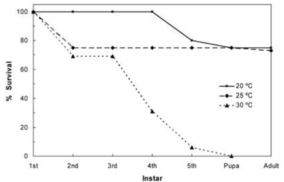
Fig. 1. Survival of Metriorhynchus elator immatures at different temperatures.
