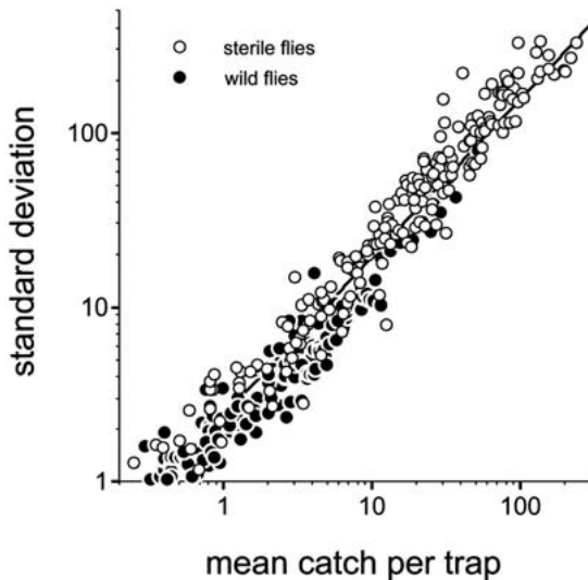
Fig. 1. The relation of standard deviation (SD) to mean ( m ) for weekly trap catches of wild and sterile Bactrocera tryoni at Gilgandra and Narrormine. The common equation \log_{10} SD = 0.37 + 0.91 \cdot (\log_{10} m) explains 91.3% of the variance of wild flies and 96.2% of that of sterile flies.
