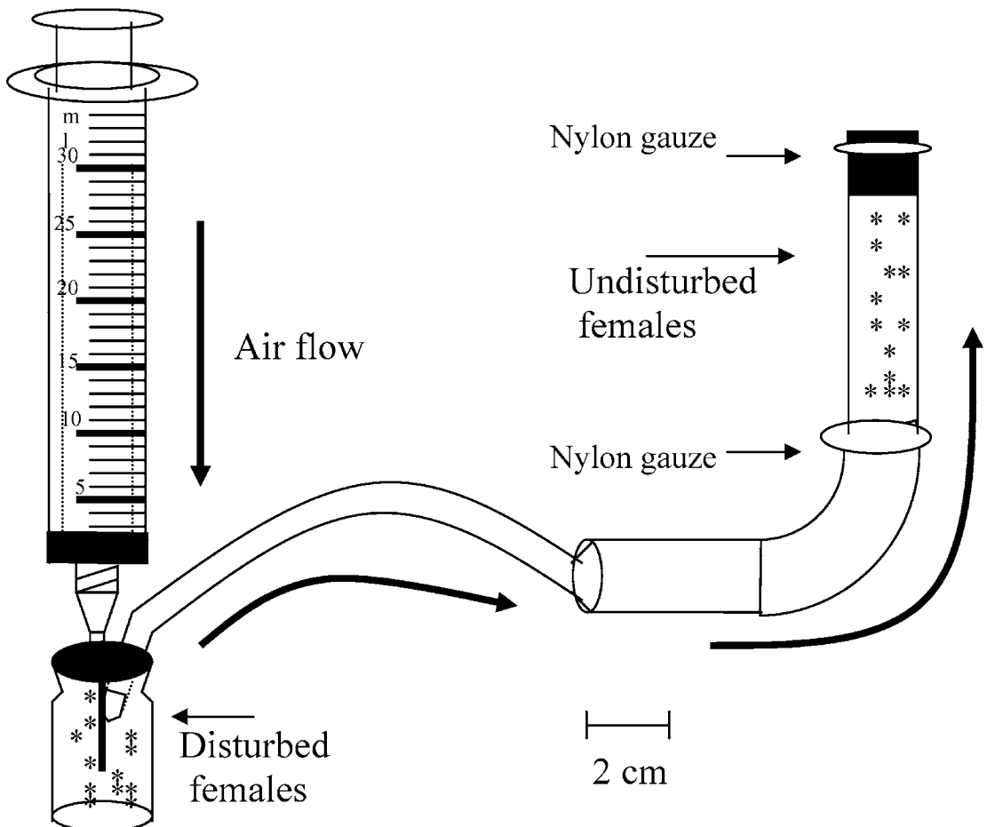
Fig. 1. Design of olfactometer used to determine the response of C. stephanoderis females to volatiles from disturbed and undisturbed insects and clean air.
