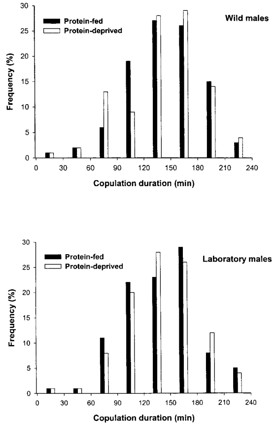
Fig. 1. Frequency distributions of duration of initial copulations between wild females and protein-fed (n = 182) and protein-deprived (n = 114) wild males (top) and protein-fed (n = 73) and protein-deprived (n = 50) mass-reared males (bottom).
