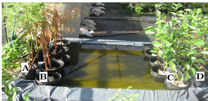
Figure 2. Bald cypress and Pond apple seedlings grown in saltwater containing 15,000 ppm sodium chloride (NaCl). A. bald cypress seedlings, 0 roots submerged but irrigated with the saltwater, survived. B. bald cypress seedlings, 100% roots submerged with the saltwater, 100% died 9 days after being treated. C. pond apple seedlings, 100% roots submerged with the saltwater, 100% growing. D. pond apple seedlings, 0 roots submerged but irrigated with the saltwater, 100% growing.
