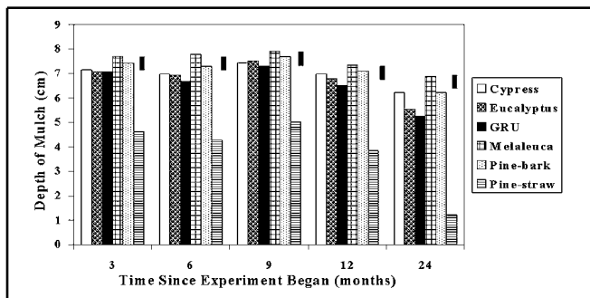
Figure 1. Settling of 6 landscape mulches (from original depth of 9 cm (3.5 in)) during the two year study.
