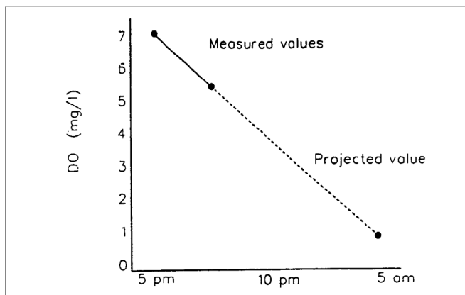
Figure 2. Estimation of potential for dissolved oxygen depletion.
