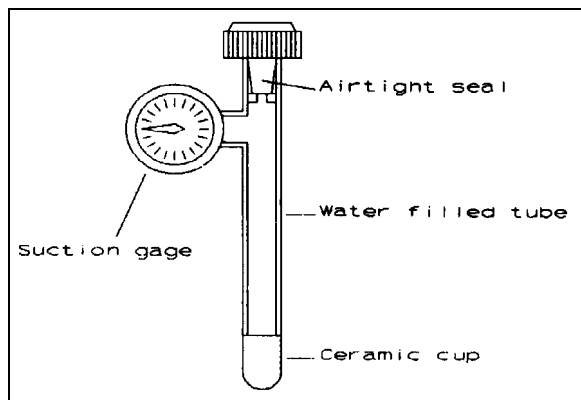
Figure 5. Tensiometer.
