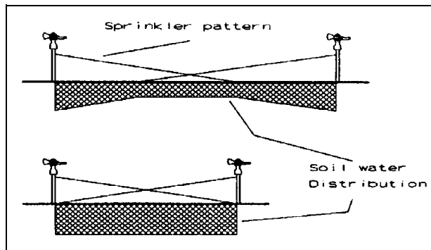
Figure 3. Water application distributions resulting from sprinkler irrigation. Excessive spacing results in a "dry" spot between sprinklers.
