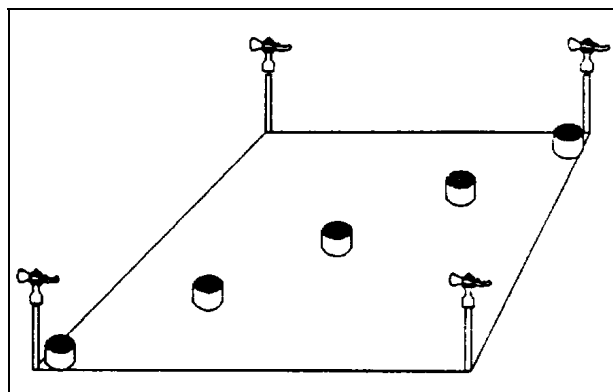
Figure 7. Test can distribution to measure application rate and uniformity.
