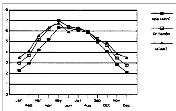
Figure 1. Inches of monthly evapotranspiration at different locations in Florida.
