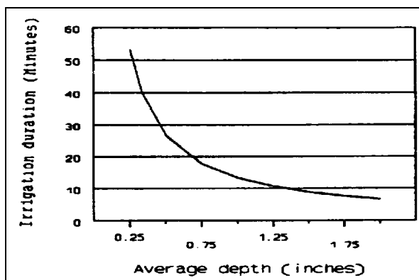
Figure 8. Time that an irrigation system should be on to apply 2/3 of an inch of water to a soil that has been depleted 50%.
