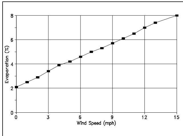
Figure 7. Sensitivity of evaporation percentage to changes in wind speed for a 5/16-inch nozzle diameter, 45 psi, and June climate data at Gainesville, FL.
