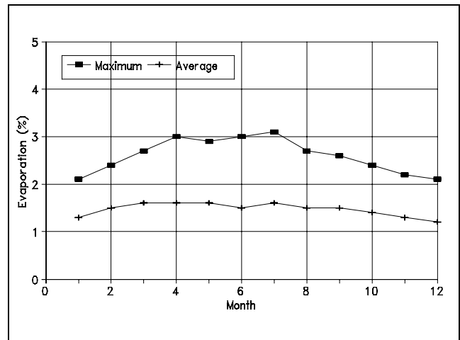
Figure 4. Maximum and average evaporation percentages for a 5/16-inch sprinkler nozzle diameter and operating pressure of 45 psi at Gainesville, FL.
