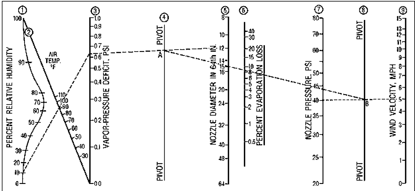
Figure 1. Sprinkler evaporation nomograph (from Frost and Schwalen, 1955).
