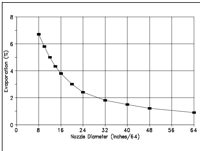
Figure 5. Sensitivity of evaporation percentage to changes in sprinkler nozzle diameter for an operating pressure of 45 psi and June climate data at Gainesville, FL.
