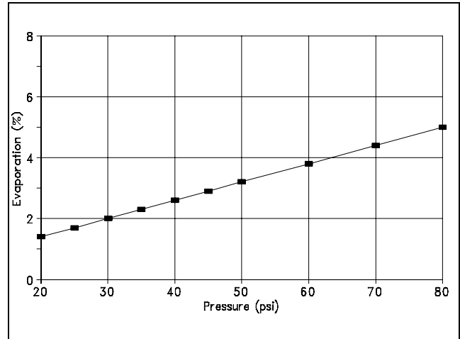
Figure 6. Sensitivity of evaporation percentage to changes in sprinkler operating pressure for a 5/16-inch nozzle diameter and June climate data at Gainesville, FL.
