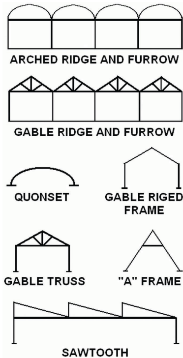
Figure 1. Greenhouse Frames
