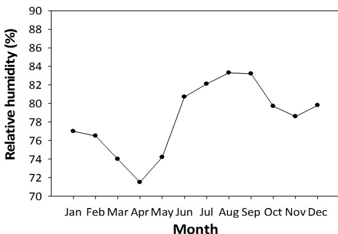
Figure 1. Monthly average air relative humidity during a 10-year period (2002-12) for southwest Florida
