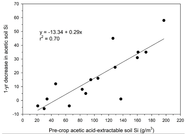
Figure 2. One-year decrease in acetic acid-extractable soil Si related to pre-crop extractable Si using treatment means for Si trials on sand soils.
