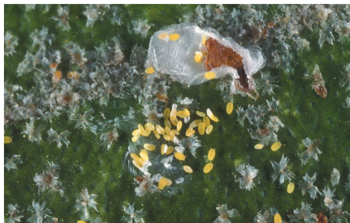
Figure 5. False oleander scale, Pseudaulacaspis cockerelli , crawlers and eggs from underneath an adult female. Credits: Lyle Buss, University of Florida
