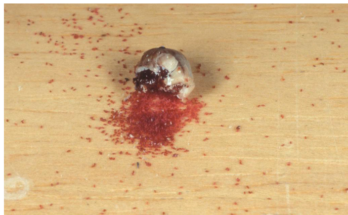
Figure 6. Barnacle scale, Ceroplastes cirripediformis , adult female ovisac and eggs. Credits: Lyle Buss, University of Florida
