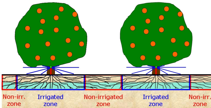
Figure 5. The citrus grove several days later, after half of the available water has been removed from the root zone. Note that water extraction has occurred from both the irrigated and non-irrigated zones.
