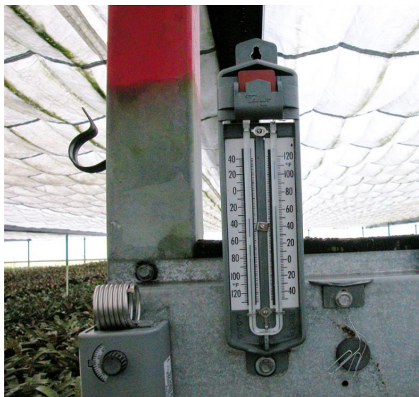
Figure 1. Retractable heat (thermal) curtain deployed under the roof in a shadehouse (Credit: Robert H. Stamps)
