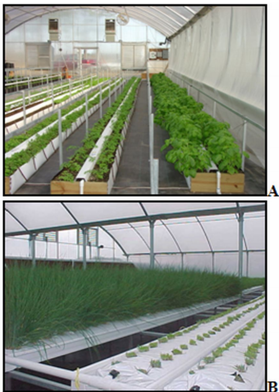
Figure 8. These photos -- taken in a greenhouse in McAlpin, FL, in 2006 -- picture (A) a crop of mixed herbs for fresh-cut, grown in an open trough filled with a peat-based mix and (B) a chives crop in perlite bags in a trough.
