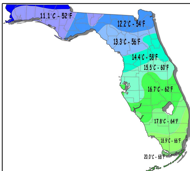
Figure 1. Average January Temperatures in Florida.
