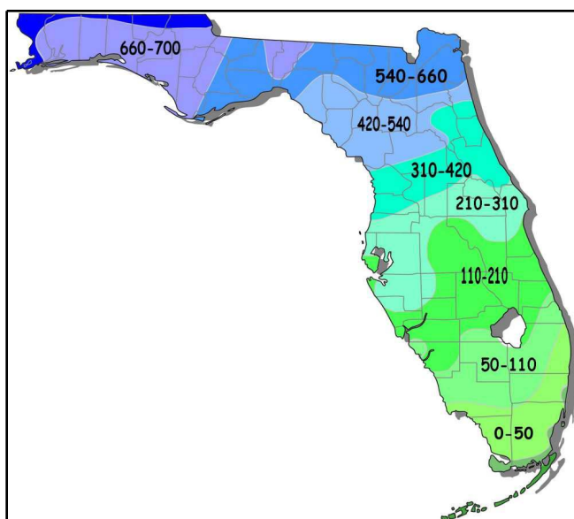
Figure 2. Estimated Chill Unit Accumulation for Florida.
