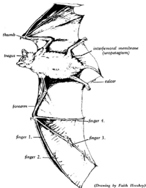
Figure 1. Bat wing structure
