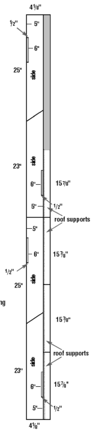
FIGURE 4 Four-chamber Nursery House Assembly Diagrams
