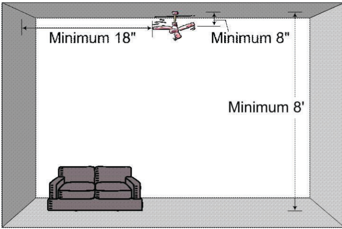
Figure 1. Minimum space requirements for a ceiling fan installation recommended by the US Department of Energy. Credits: Image created by Hyun-Jeong Lee in Microsoft Office Visio. Converted to .GIF by UF/IFAS Communication
