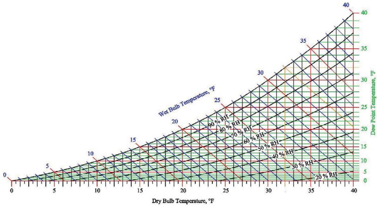
Figure 1. Psychrometric Chart.
