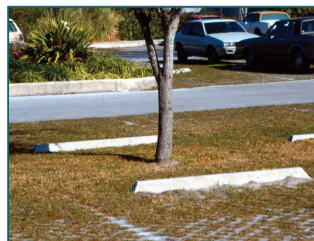
Consider soil properties (soil depth, water table and compaction). This porous surface reduces runoff and improves root health.
