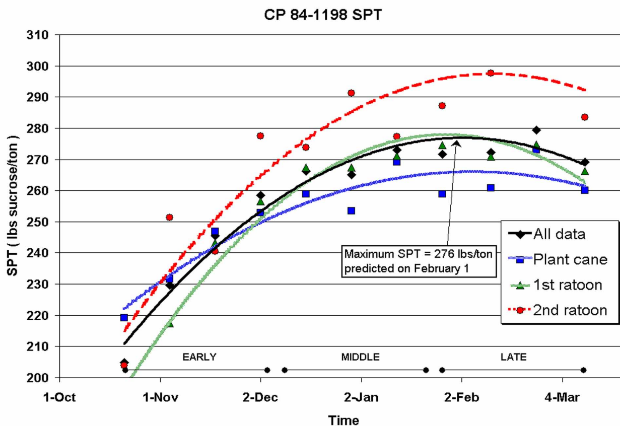
Figure 1. Sucrose Accumulation Maturity Curves for CP 84-1198.
