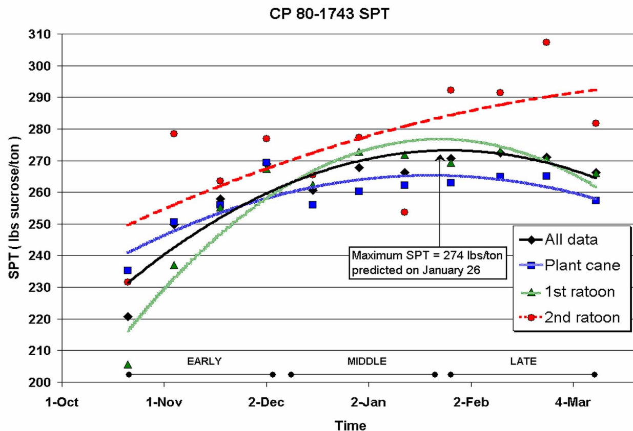
Figure 1. Sucrose Accumulation Maturity Curves for CP 80-1743.
