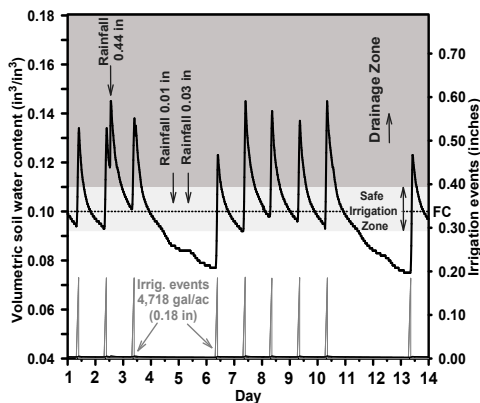
Figure 2. Example of excessive (“over”) irrigation of the upper soil layer (0 to 6 inch depth) moisture content for drip irrigation under plastic mulched condition for sandy soils. Black line indicates volumetric soil water content using soil moisture sensors. Grey line indicates Irrigation event, single daily irrigation event with volume application of 65 gal/100ft (0.18 in). Dotted line indicates soil field capacity line. Arrows indicate rainfall events.
