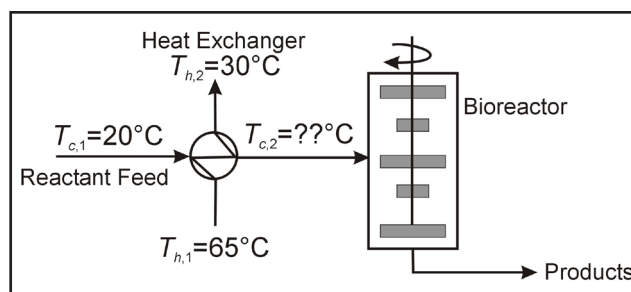
Figure 1. Process flow diagram of the feed preheater and bioreactor.
