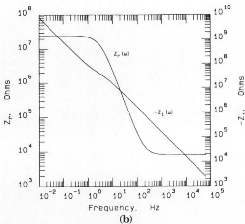
FIGURE 6. Impedance data for a system consisting of a resistor in series with the parallel combination of a capacitor and a resistor and capacitor in series: a) impedance plane plots with frequency as a parameter; b) Bode plots for real and imaginary components of impedance.
