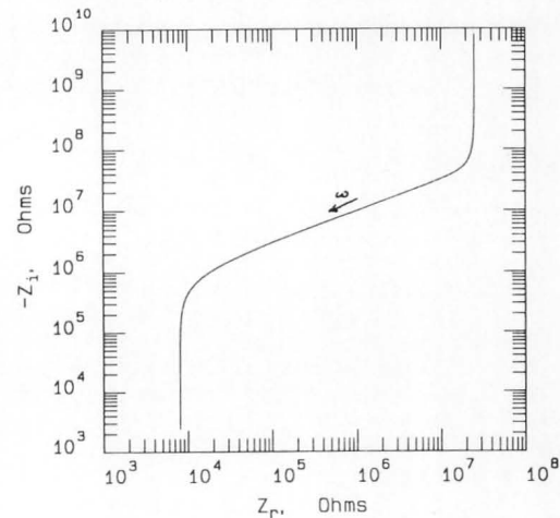
FIGURE 7. Impedance data for the system of Figure 6 consisting of a resistor in series with the parallel combination of a capacitor and a resistor and capacitor in series.
