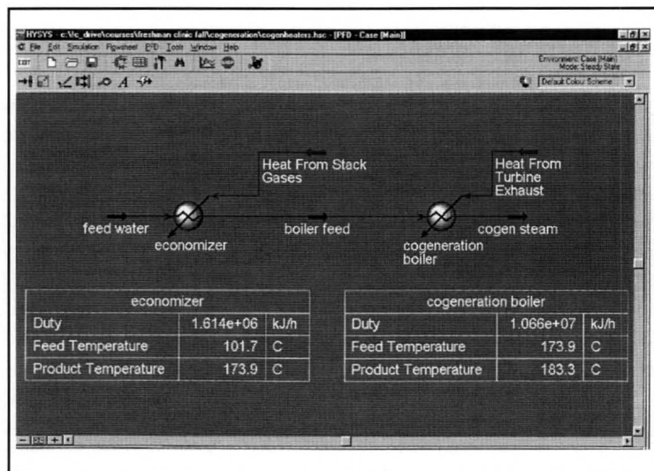
Figure 4. HYSYS-generated process flow diagram with summary tables.
