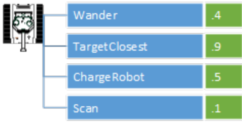
Figure 1: A composite robot behavior in RoboCodePlus. Each behavior (blue rectangle) is associated with a weight (green rectangle) which determines its precedence in the Priority Fusion arbiter.
